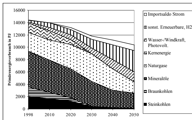
Fig. 2: RRO-IER: renewables and efficient energy technologies scenario, primary energy demand in PJ
