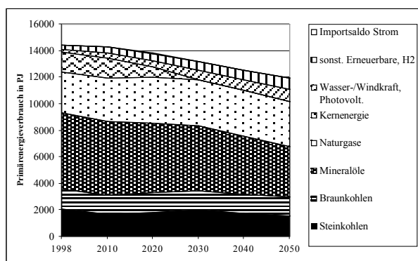
Fig. 1: REF-IER: reference scenario, primary energy demand in PJ
