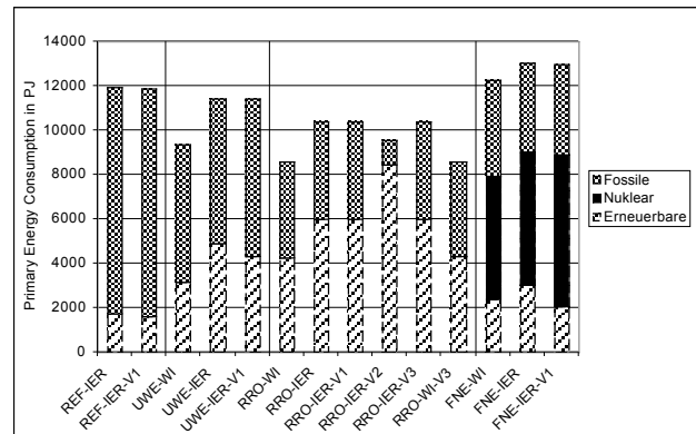
Fig. 4: Primary Energy Consumption by the Year 2050, According to the various scenarios 2
