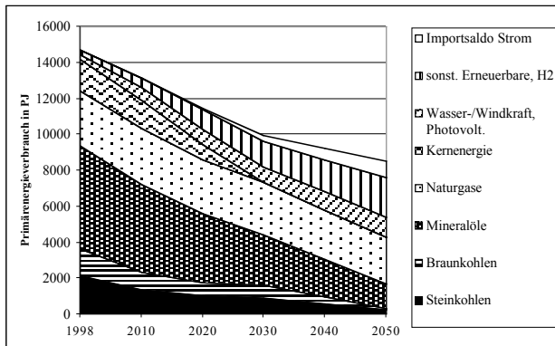
Fig.3: RRO-WI: renewables and efficient energy technologies scenario, primary energy demand in PJ
